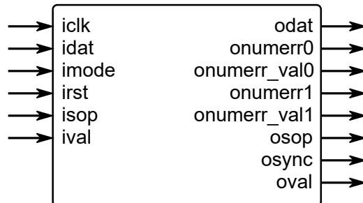
Figure 4. The I.6 40G LDPC Decoder port map
